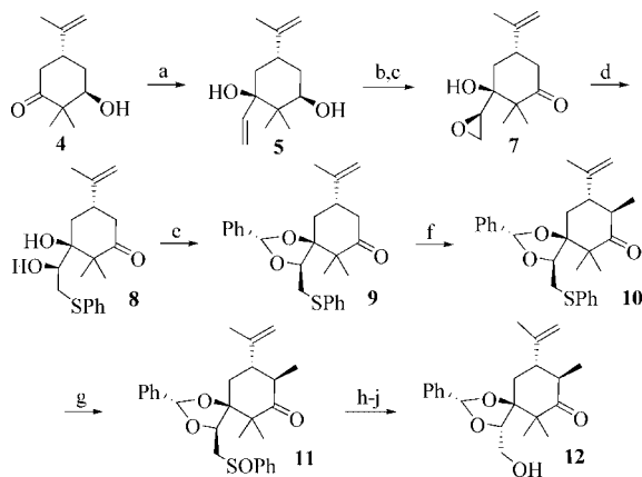
Scheme 3. (a) Tetravinylltin, BuLi, THF, -78^{\circ}\text{C} , 96%; (b) VO(acac) 2 , t BuOOH, CH 2 Cl 2 ; (c) Jones reagent, acetone, 60% over 2 steps; (d) K 2 CO 3 , PhSH, CH 3 CN, 91%; (e) PhCH(OMe) 2 , NSA, CH 2 Cl 2 , 92%; (f) t BuOK, MeI, THF, 97%; (g) NaIO 4 , MeOH, 94%; (h) (CF 3 CO) 2 O, pyridine, THF, 0^{\circ}\text{C} ; (i) K 2 CO 3 , H 2 O; (j) LiAlH(OCMe 3 ) 3 , THF, 0^{\circ}\text{C} , 81% overall.
