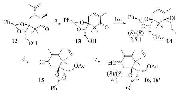
Scheme 4. (a) O 3 , MeOH, -78^{\circ}\text{C} , Cu(OAc) 2 , FeSO 4 , 77%; (b) allyl Grignard reagent, THF, 0^{\circ}\text{C} ; (c) Ac 2 O, NEt 3 , CH 2 Cl 2 , 90% over 2 steps; (d) SOCl 2 , CH 2 Cl 2 , -20^{\circ}\text{C} ; (e) Al 2 O 5 , 71% over 2 steps.
