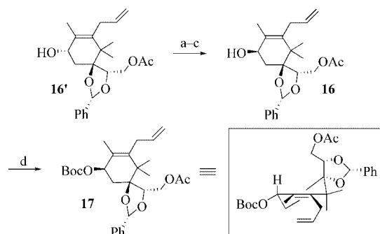
Scheme 5. Conversion of 16' into 16 and formation of 17 . (a) PPh 3 , DIAD, PhCOOH, THF; (b) K 2 CO 3 , MeOH; (c) Ac 2 O, NEt 3 , CH 2 Cl 2 , 52% overall; (d) DMAP, Boc 2 O, CH 3 CN, 61%.
