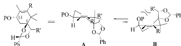
Scheme 1. Stability of half chair of ring A with Taxol stereochemistry.
