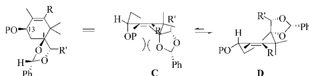
Scheme 2. Stability of half chair of ring A with Taxol epimeric stereochemistry.
