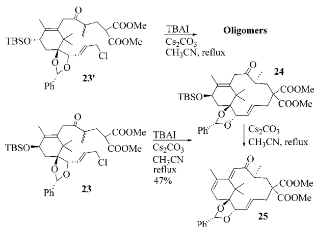
Scheme 7. Attempts of macrocyclization on two different diastereoisomers.
