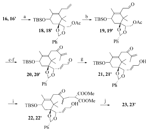
Scheme 6. Synthesis of 23 and 23' . (a) TBDMSCl, imidazole, DMF, 92%; (b) \text{O}_3 , MeOH, \text{PPh}_3 , -78^\circ\text{C} , 88%; (c) \text{CH}_2=\text{C}(\text{CH}_3)\text{-MgBr} , THF, -78^\circ\text{C} ; (d) \text{K}_2\text{CO}_3 , MeOH; (e) Dess–Martin periodinane, \text{CH}_2\text{Cl}_2 ; (f) \text{PPh}_3=\text{CH}(\text{CHO}) , toluene, 55% overall; (g) \text{LiAlH}(\text{OC}_2\text{H}_5)_3 , THF, -78^\circ\text{C} , 87%; (i) dimethyl malonate, \text{Cs}_2\text{CO}_3 , \text{CH}_3\text{CN} , 86%; (j) (\text{CH}_3)_2\text{NCCl}=\text{C}(\text{CH}_3)_2 , \text{CH}_2\text{Cl}_2 , 91%.
